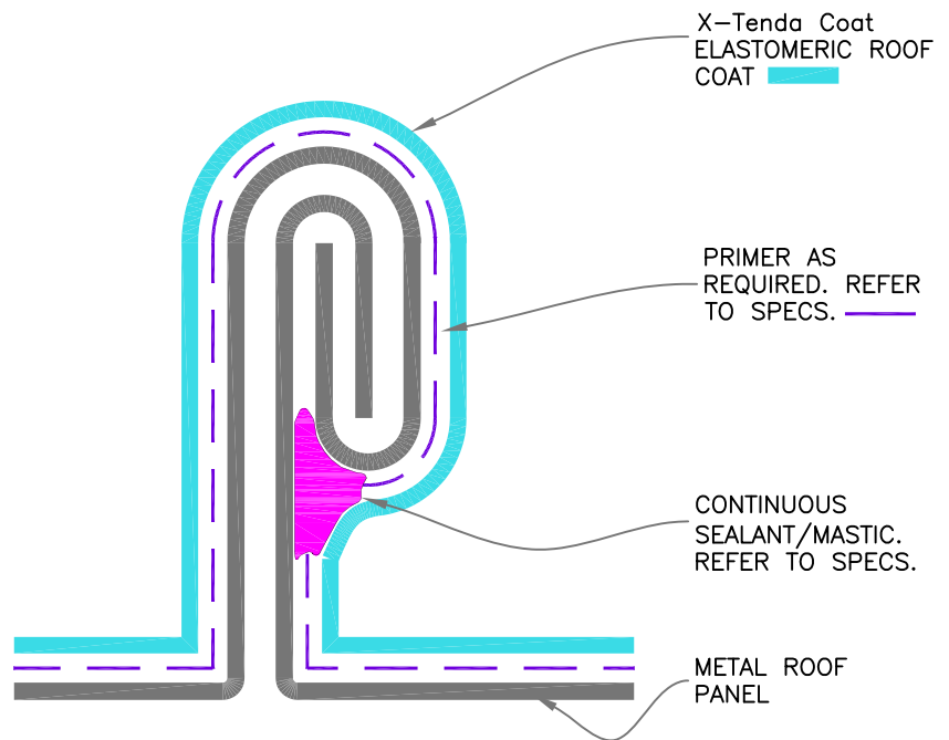
B: COATING DETAIL AT STANDING SEAM
