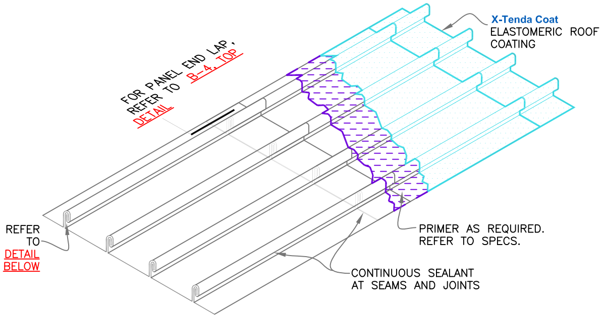
A: 3D VIEW OF TYPICAL METAL ROOF
