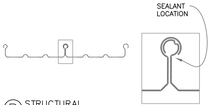
(B) STRUCTURAL STANDING SEAM ROOF
