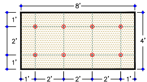
FIG. 3: A-27B (55MPH WARRANTY WIND SPEED)
