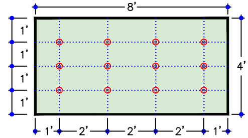
FIG. 1: A-27D (55 OR 72MPH WARRANTY WIND SPEED)
