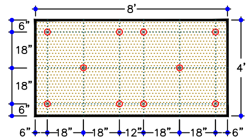
FIG. 2: A-27C (72MPH WARRANTY WIND SPEED)
