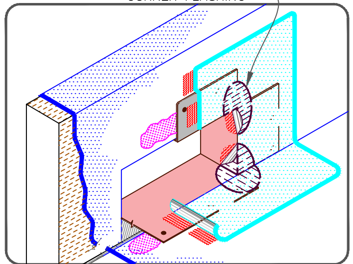
TPO PRE-MOLDED OUTSIDE CORNER FLASHING
