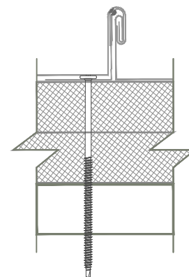
CROSS SECTION 180° SEAMING
