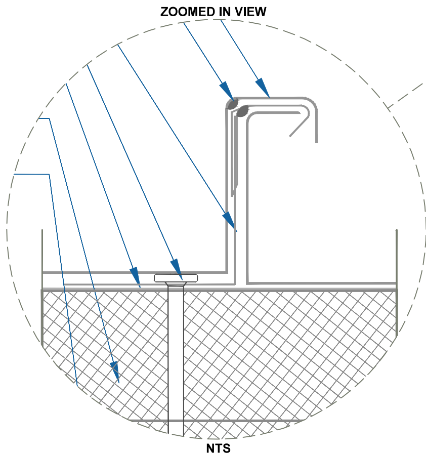
CROSS SECTION BEFORE SEAMING
