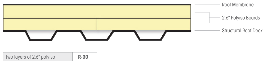
Option #1 - R-30ci Roof Assembly
