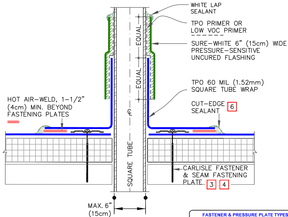
FASTENER & PRESSURE PLATE TYPES FOR DIFFERENT ROOF DECKS
