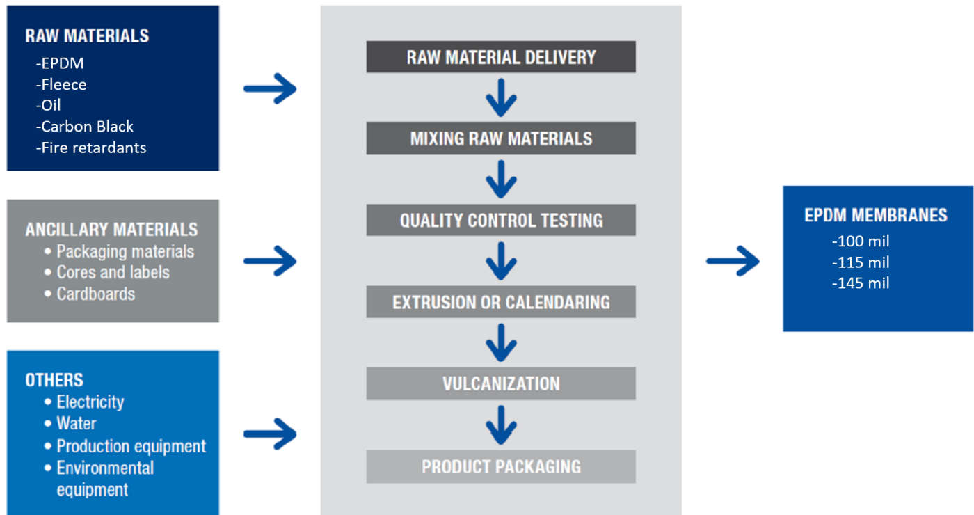
Figure 1: FleeceBACK® EPDM production process map
