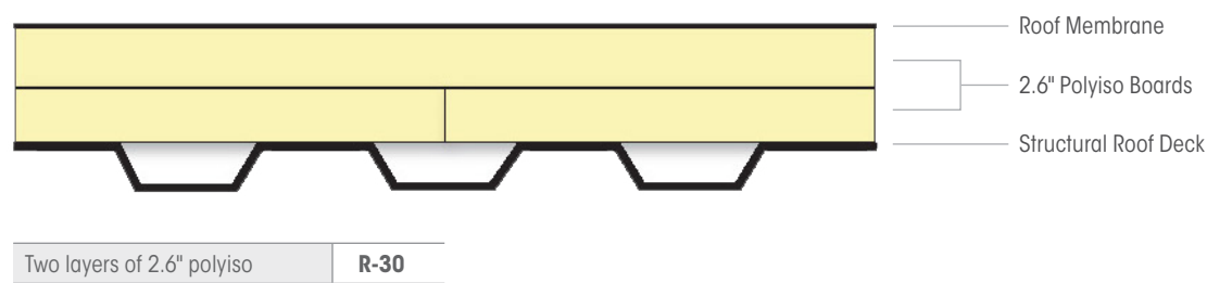
Option #1 - R-30ci Roof Assembly
