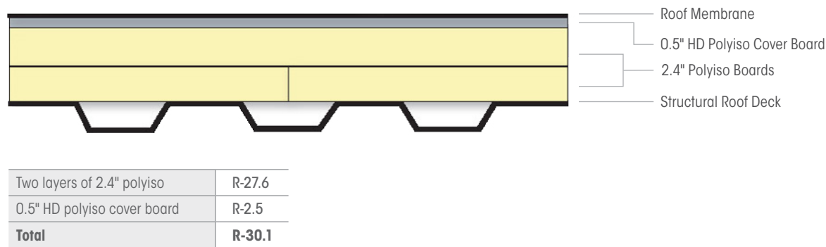
Option #2 - R-30ci Roof Assembly
