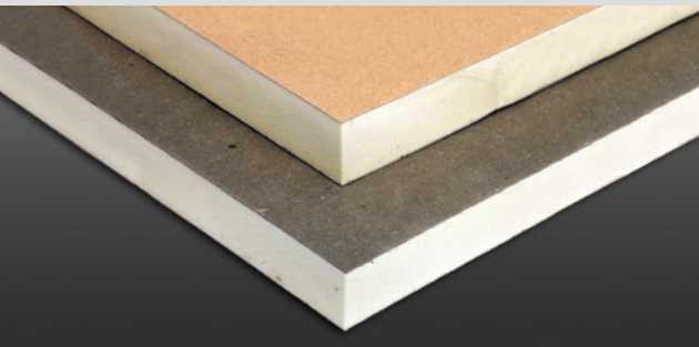
Light- and dark-colored glass reinforced felt (GRF) facers
