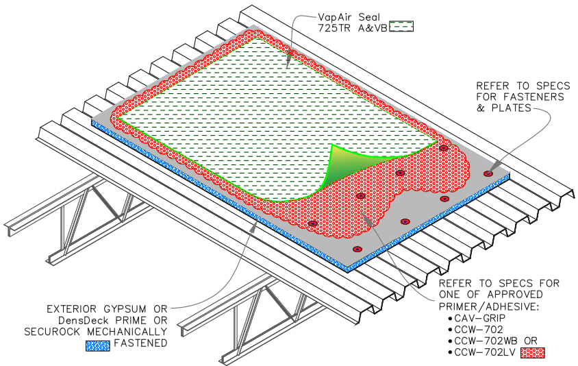
B 3-D VIEW OF TYPICAL ROOF ASSEMBLY
