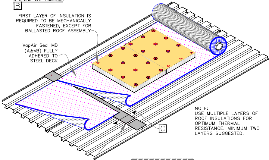
3-D END-LAP ASSEMBLY
