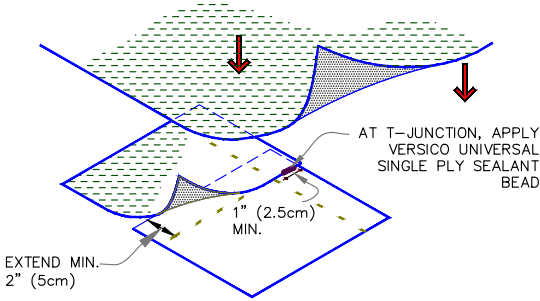
C T-JUNCTION OF SEAMS WITH SEALANT
