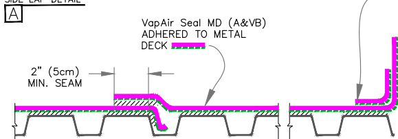
SIDE LAP DETAIL
