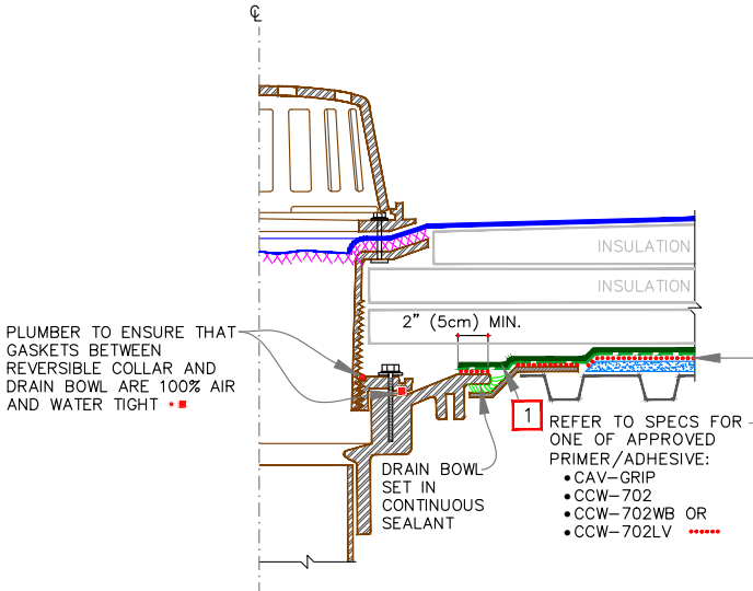
ADJUSTABLE DRAIN – TYPE A
