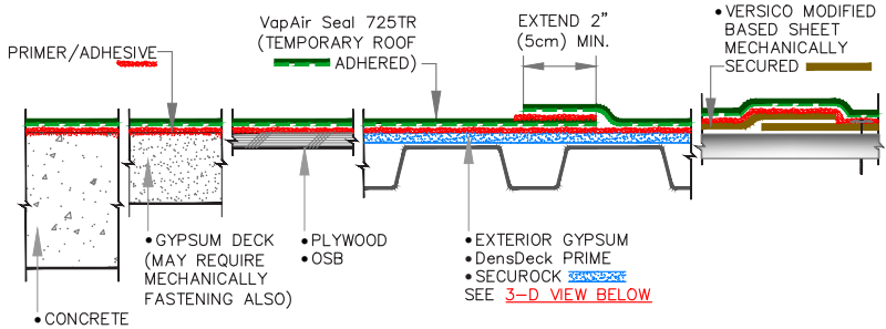
A APPLICABLE SUBSTRATES & SEAM DETAIL
