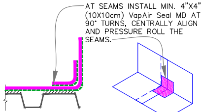
ROOF TO WALL TRANSITION
