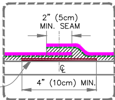
SEAM CROSS-SECTION
