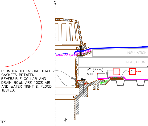
EXAMPLE OF ADJUSTABLE DRAIN - TYPE A
