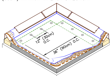
CORNER REINFORCEMENT
