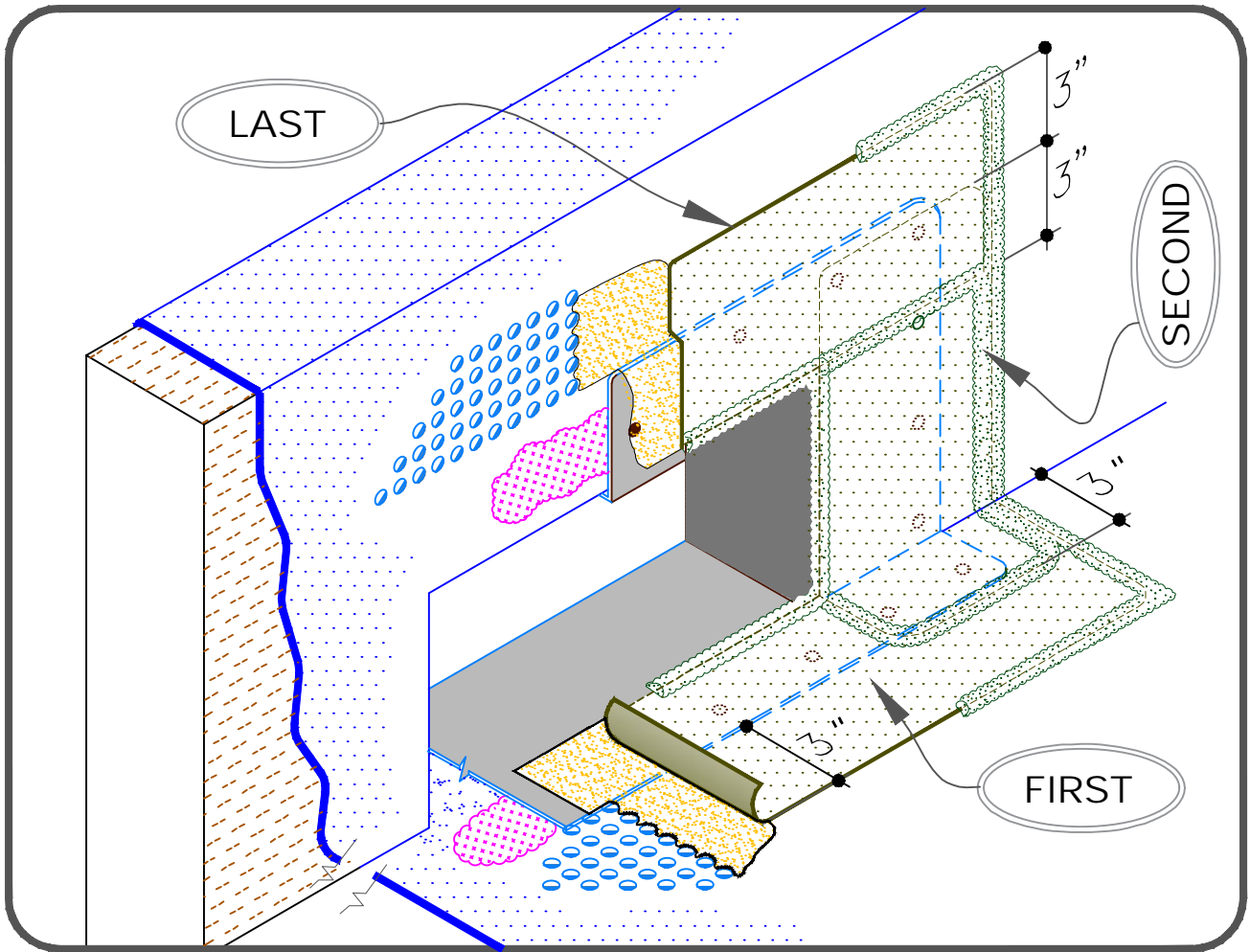
ISOMETRIC
