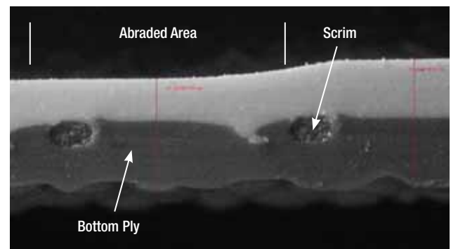
Membrane: 60-mil PVC Beginning Thickness: 58.94 Ending Thickness: 50.81
