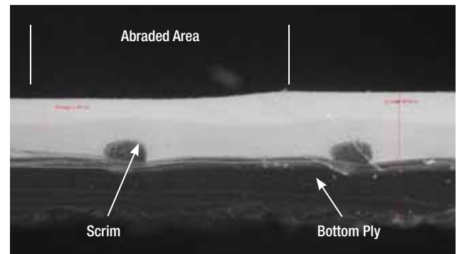
Membrane: 60-mil PVC Beginning Thickness: 59.77 Ending Thickness: 54.81
