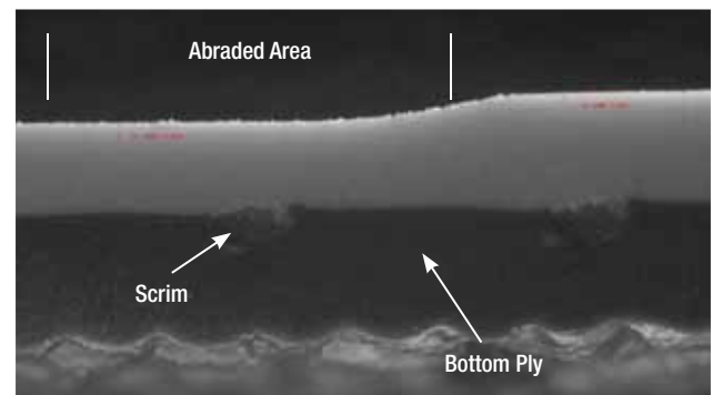
Membrane: 80-mil PVC Beginning Thickness: 78.58 Ending Thickness: 73.57
