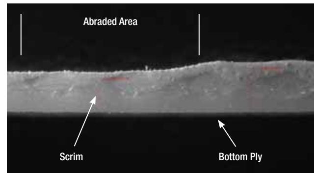
Membrane: 36-mil PVC/KEE Beginning Thickness: 32.74 Ending Thickness: 27.37
