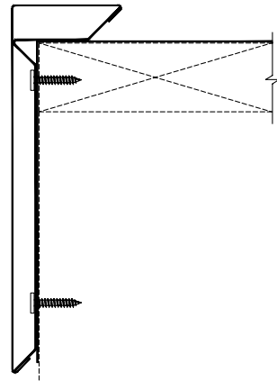
Fascia
