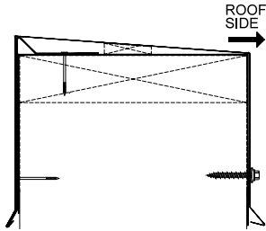
Coping
