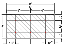
(B) FIELD OF ROOF 6 FASTENERS PER 4'X8' BOARD
