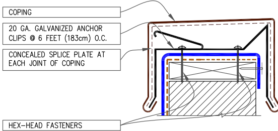
9F SecurEdge 200 & 300 COPING
