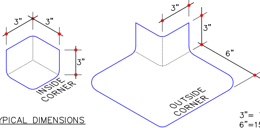
TYPICAL DIMENSIONS
