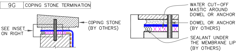
9G COPING STONE TERMINATION
