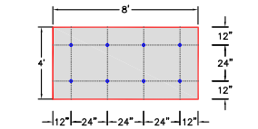
(A) PERIMETER ZONE 8 FASTENERS PER 4'X8' BOARD
