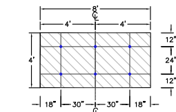
(B) FIELD OF ROOF 6 FASTENERS PER 4'X8' BOARD
