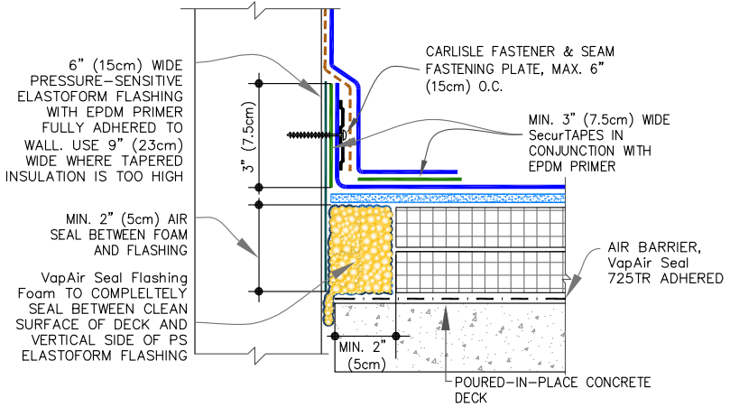
(A) OPTION: AIR SEALING WITH FOAM
