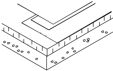
MEMBRANE SPLICE WITH QA SEAM TAPE (FOR QA SEAM TAPE INTERSECTIONS, REFER TO VERSICO DETAIL C-2.2)
