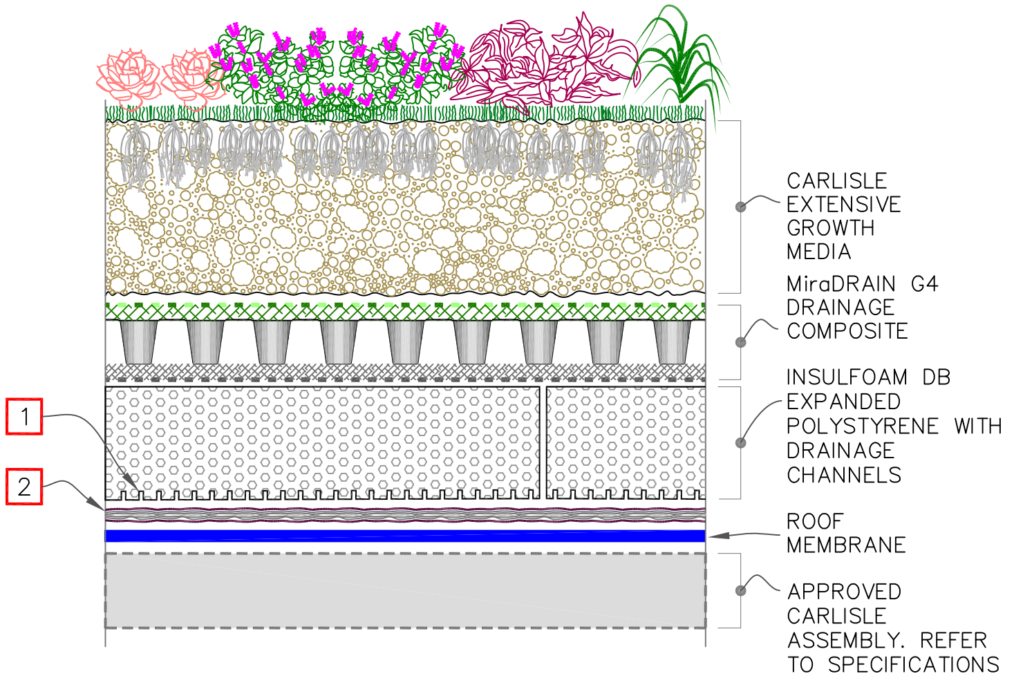
CARLISLE ROOF GARDEN EDGE PER RG U-1.1A , RG U-1.1B & SPECS.
