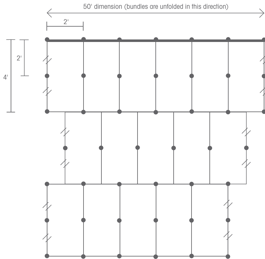
Figure 1 Fastening Pattern for GreenGuard PB6 Roofing Recover Boards Installed Directly Under Dark-colored Roof Membranes in Mechanically Attached and Loose-Laid and Ballasted Roof Systems. (Top view, represents only a small portion of three adjacent GreenGuard PB6 bundles are shown.)
