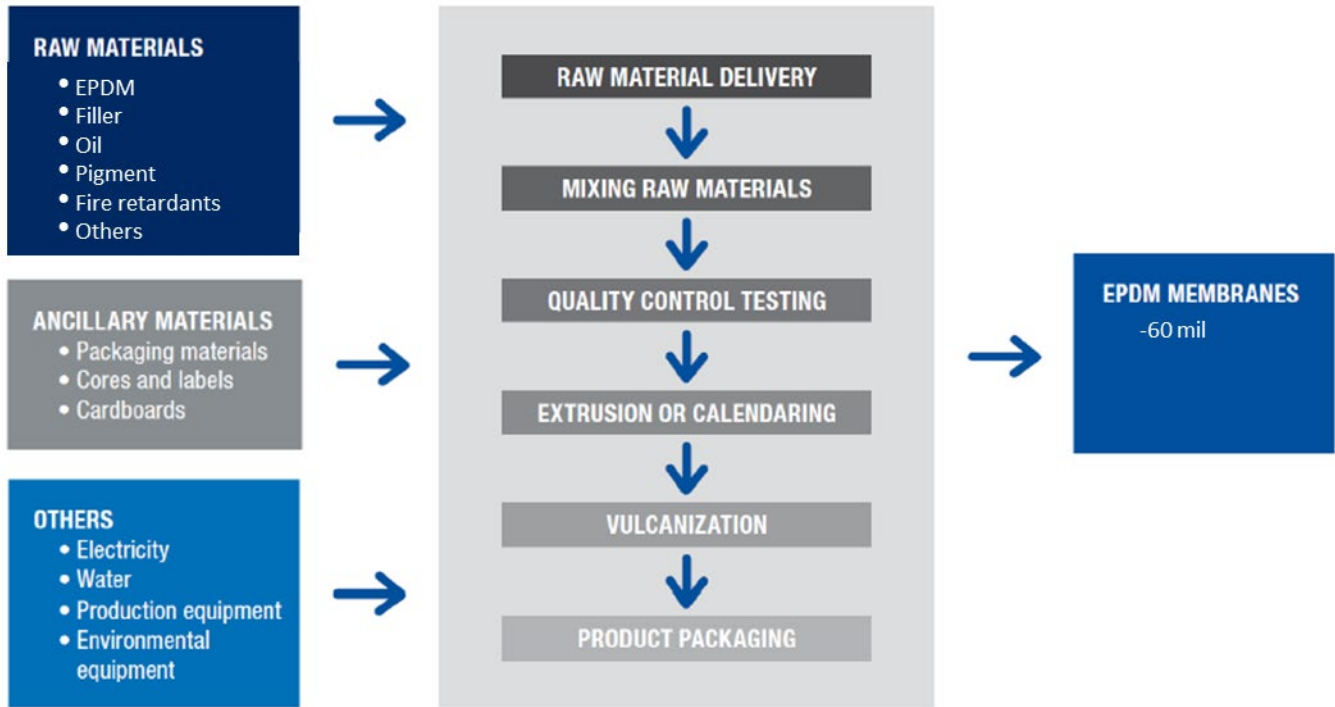
Figure 1: Sure-White® SAT™ Non-Reinforced EPDM production process map
